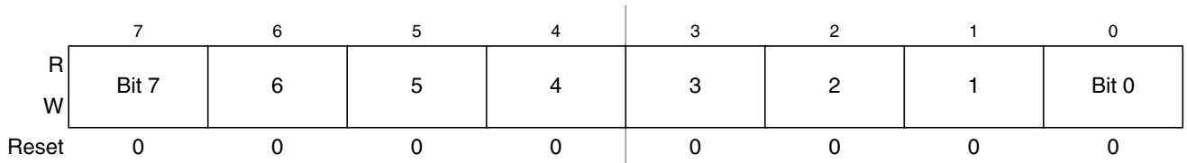
Figure 12-24. PWM Channel Period Registers (PWMPER3)
