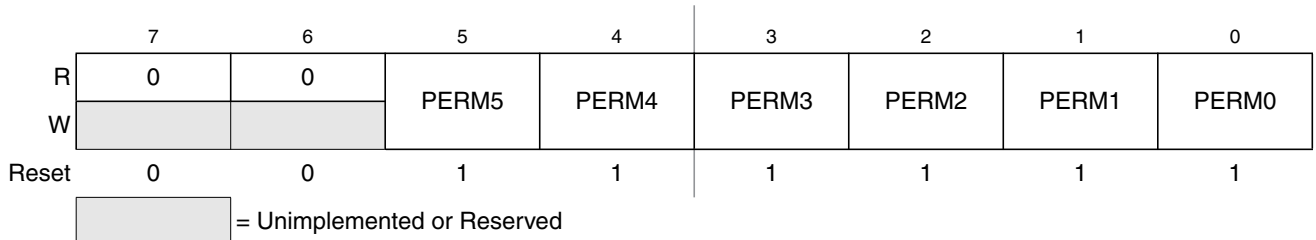
Figure 2-21. Port M Pull Device Enable Register (PERM)
