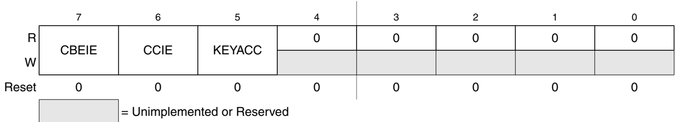
Figure 17-7. Flash Configuration Register (FCNFG)
