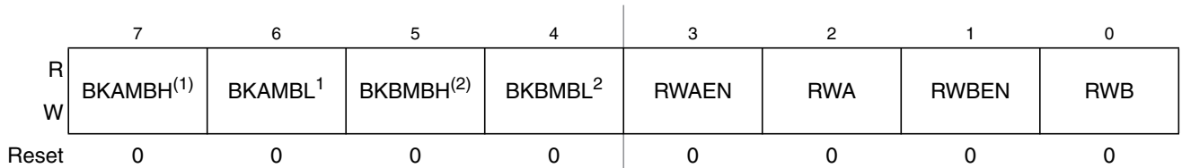
Figure 7-14. Debug Control Register 3 (DBGC3)
