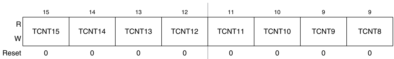
Figure 15-10. Timer Count Register High (TCNTH)
