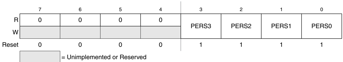
Figure 2-14. Port S Pull Device Enable Register (PERS)
