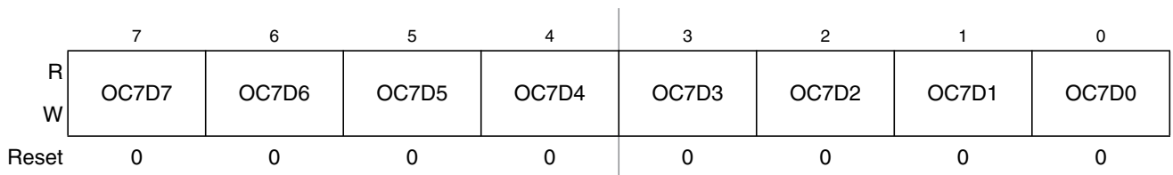
Figure 15-9. Output Compare 7 Data Register (OC7D)
