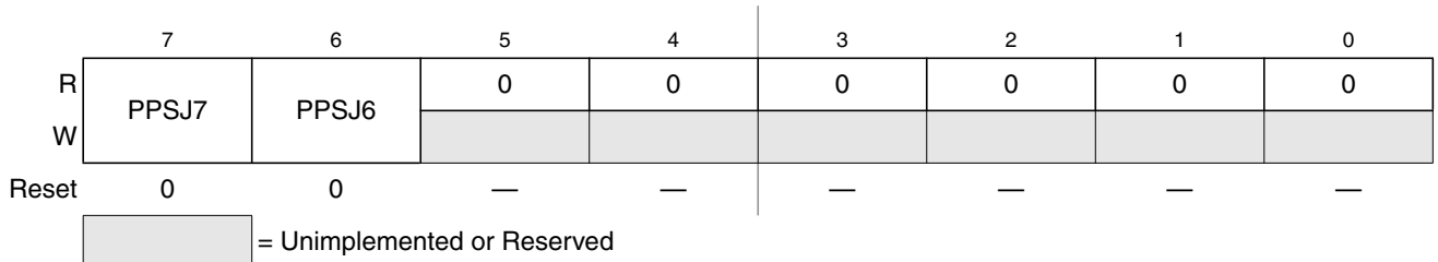
Figure 2-37. Port J Polarity Select Register (PPSJ)
