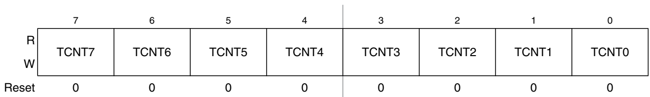
Figure 15-11. Timer Count Register Low (TCNTL)
