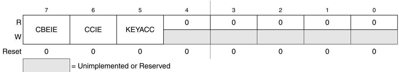
Figure 20-7. Flash Configuration Register (FCNFG)
