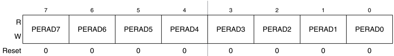
Figure 2-44. Port AD Pull Device Enable Register (PERAD)
